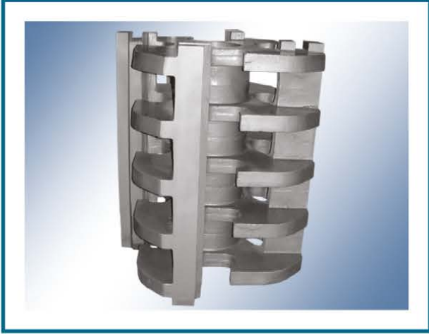
Rotor (2460 kg)
