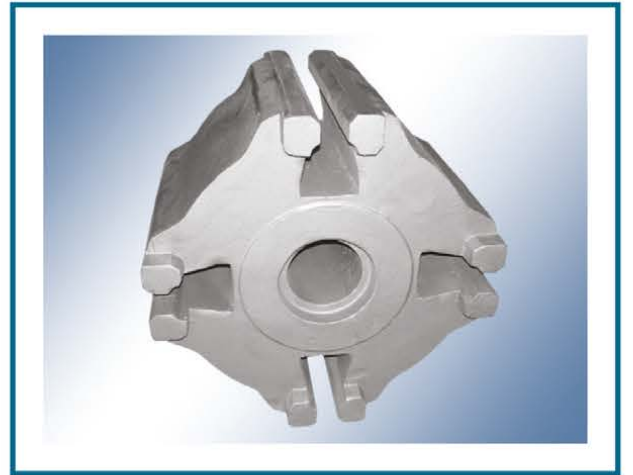
Rotor (4750 kg)
